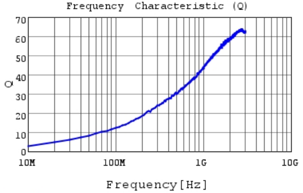
LQG18HH2N2S00 Q
