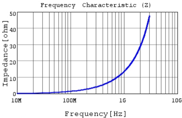
LQG18HH2N2S00 |Z|
