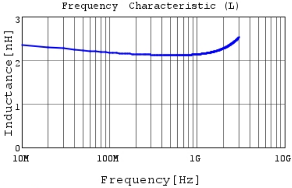
LQG18HH2N2S00 L
