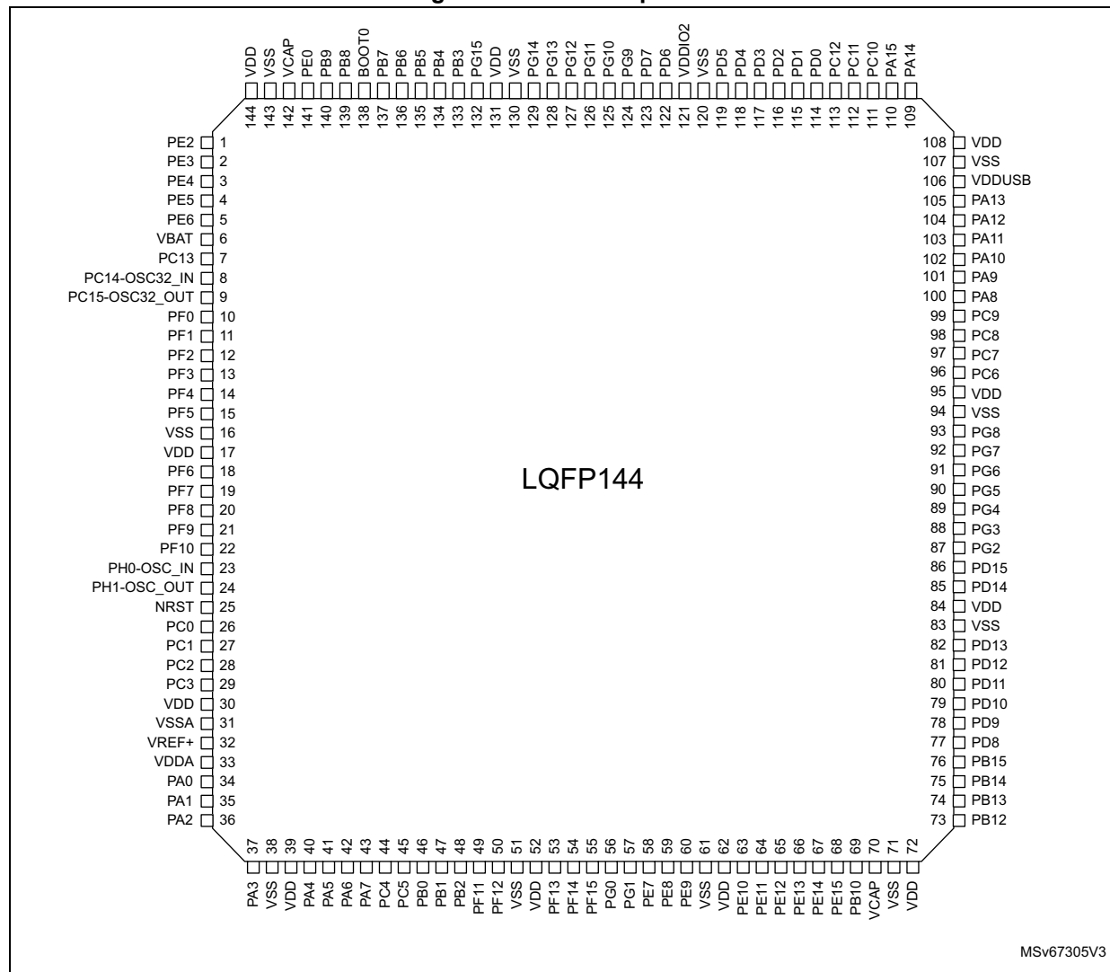
Figure 10. LQFP144 pinout
