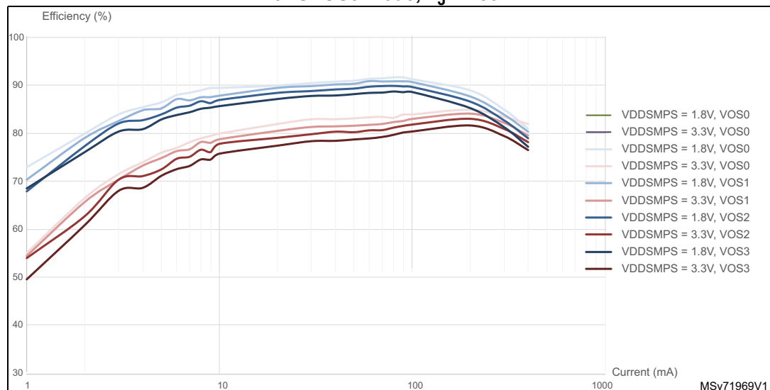
Figure 24. SMPS efficiency versus load current in Run, Sleep and Stop mode with SVOS3 mode, T_J = 130^\circ\text{C}
