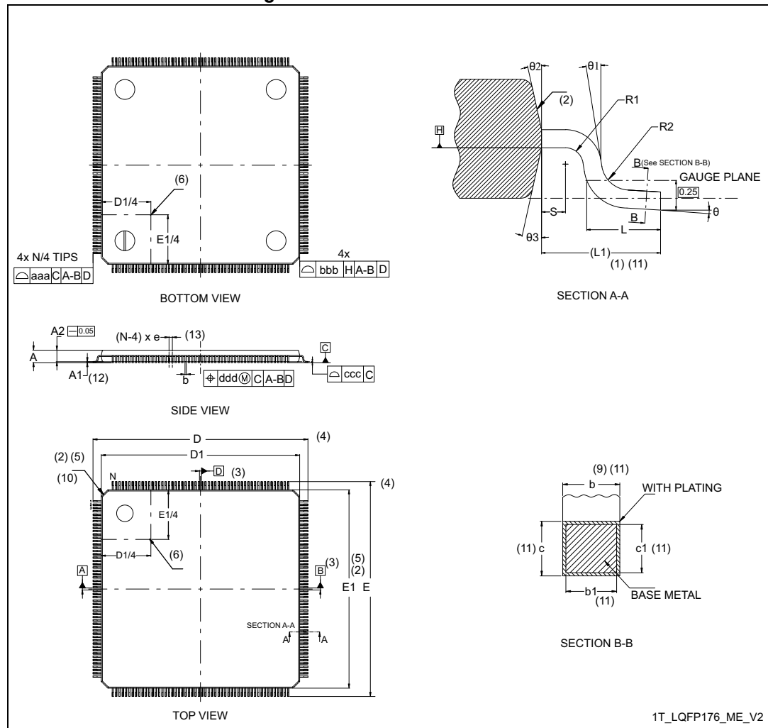
Figure 89. LQFP176 - Outline (15)
