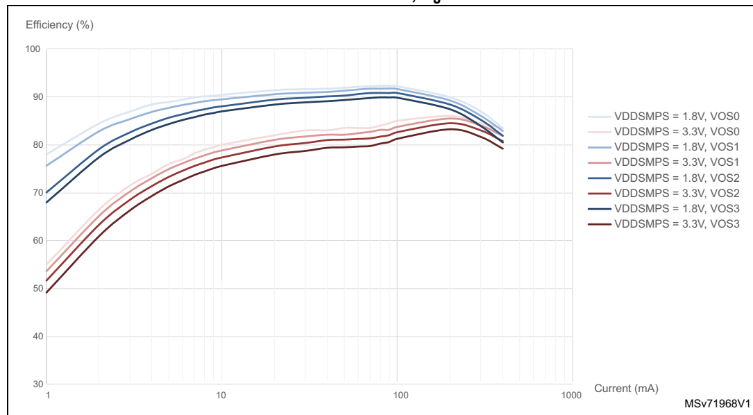
Figure 23. SMPS efficiency versus load current in run, sleep and stop mode with SVOS3 mode, T_J = 30^\circ\text{C}
