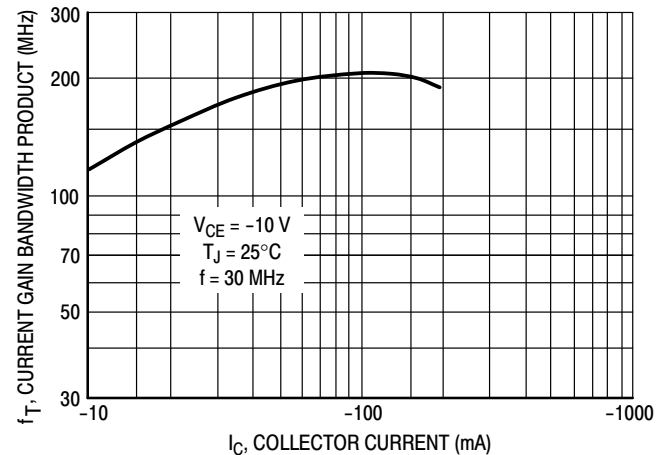
Figure 2. Current Gain Bandwidth Product
