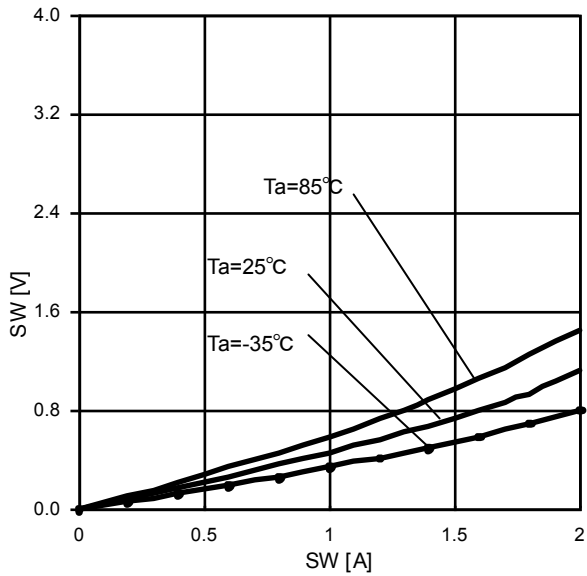
Fig.18 SAT Voltage
