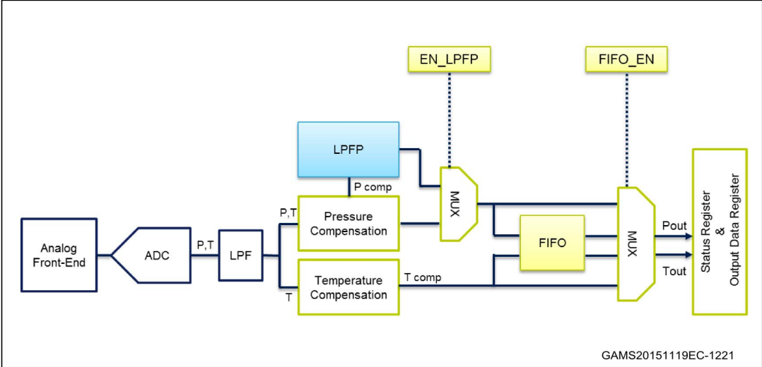
Figure 2. Digital logic
