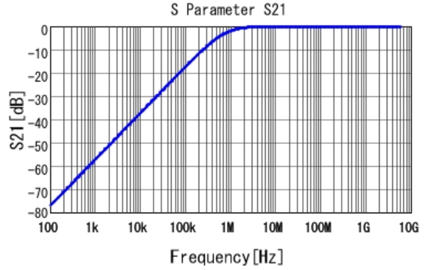
GCM155R71H222KA37 S21 DC0V, 25degC
