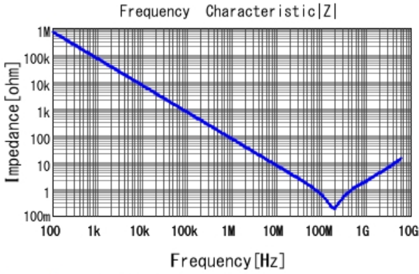
GCM155R71H222KA37 |Z| DCOV, 25degC
