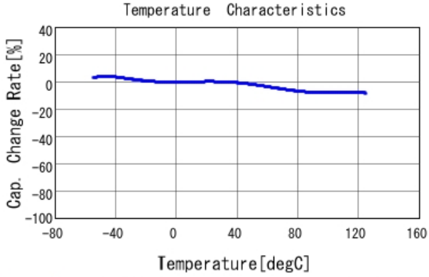
GCM155R71H222KA37 C-Temp. capchange, DC0.0V, AC1.C
