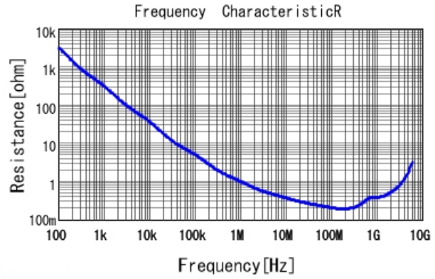
GCM155R71H222KA37 R DCOV, 25degC
