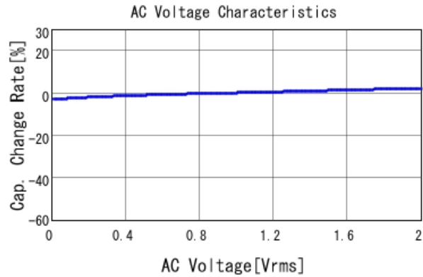
GCM155R71H222KA37 C-AC Voltage capchange, DCOV, 25
