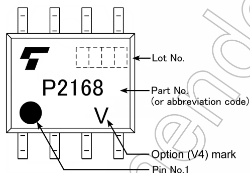
Fig. 16.3 Marking Example(Note 1)
