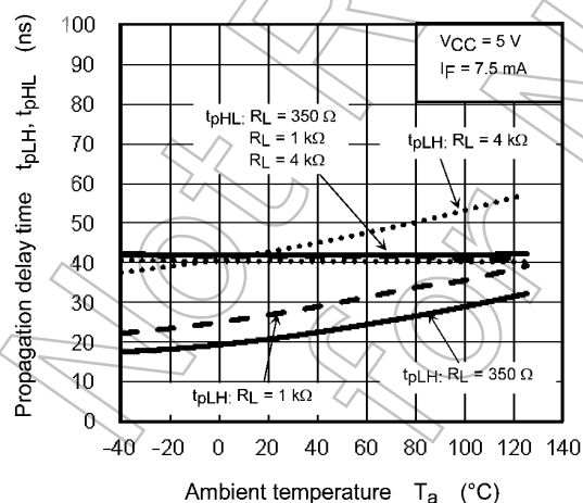
Fig. 12.2.11 t_{pLH}/t_{pHL} - T_a
