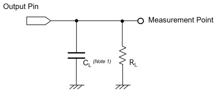
Measurement Circuit for t_{PLH} and t_{PHL}
