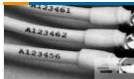
TE Part #5054212004 RNF-100-1/2-3-STK
