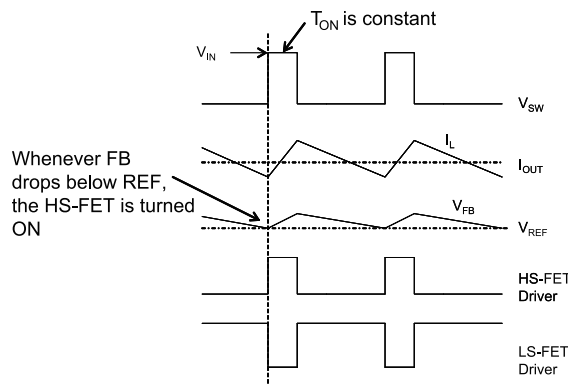
Figure 2: Heavy-Load Operation
