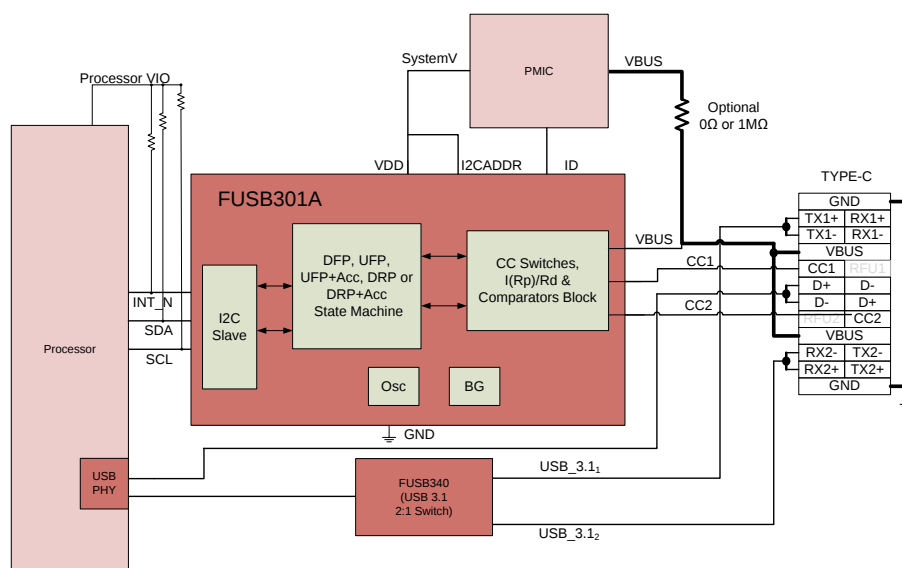
Figure 1. Typical Application
