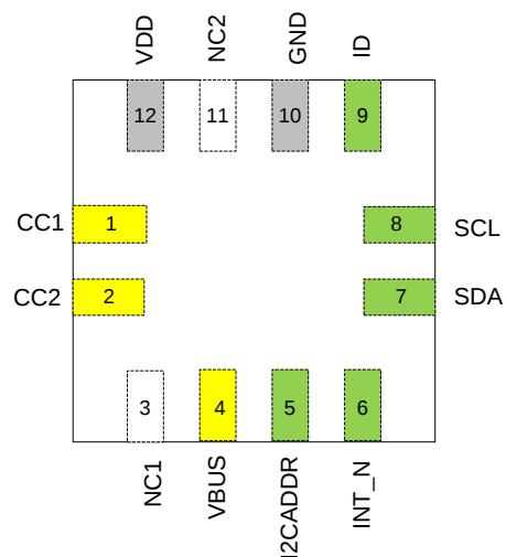
Figure 3. Pin Assignment (Top Through View)
