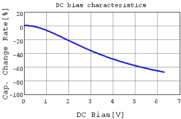
GRM188R60J475KE19 C-DC bias capchange, 25.0c
