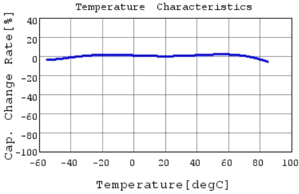
GRM188R60J475KE19 C-Temp. capchange, DC0.0V,
