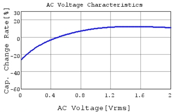
GRM188R60J475KE19 C-AC Voltage capchange, Dc
