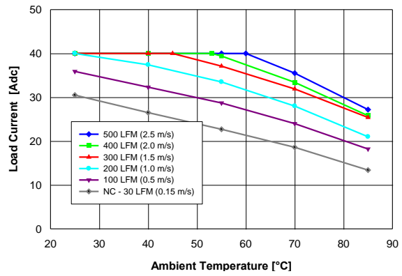
Fig. 2: Available load current vs. ambient air temperature and airflow rates for converter with G height pins mounted horizontally with air flowing from pin 1 to pin 3, MOSFET temperature \le 120^\circ\text{C} , V_{in} = 48\text{ V}
