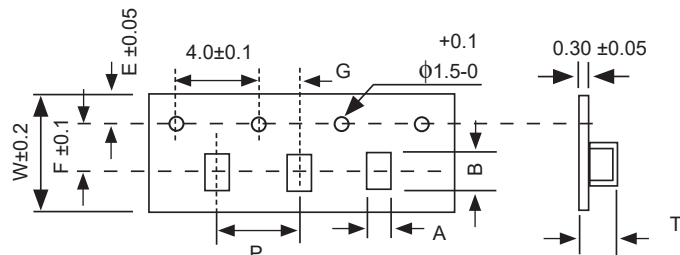
FIGURE 2 (EMBOSSED PLASTIC TAPE)
