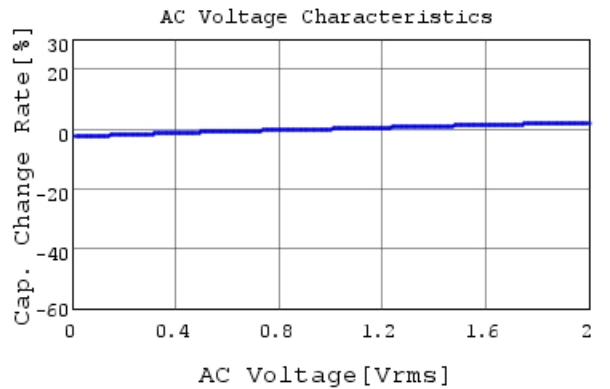
GRM188R72A104KA35 C-AC Voltage capchange, Dc
