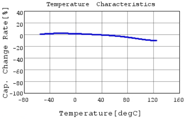
GRM188R72A104KA35 C-Temp. capchange, DC0.0V,
