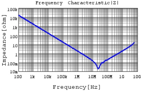
GRM188R72A104KA35 |Z| DCOV, 25degC
