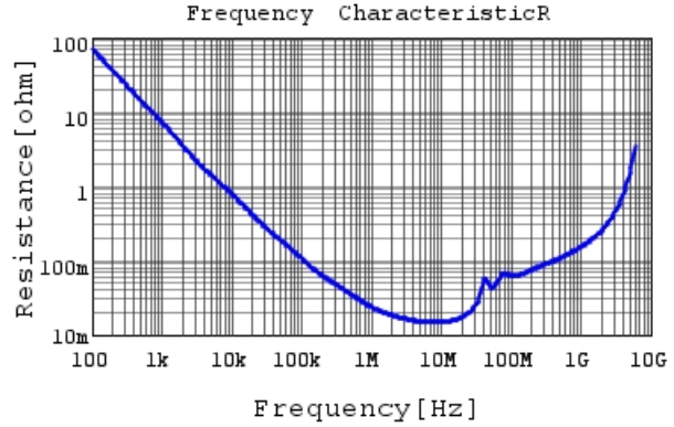
GRM188R72A104KA35 R DCOV, 25degC
