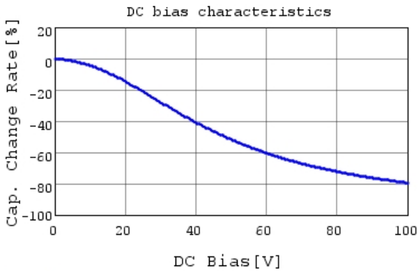
GRM188R72A104KA35 C-DC bias capchange, 25.0c
