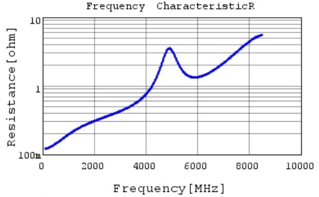
GRM1555C1H120GA01 R DCOV, 25degC
