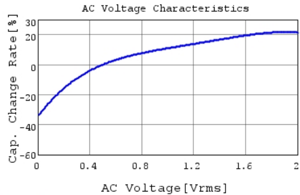
GCM31CR70J226ME23 C-AC Voltage capchange, DC
