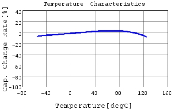
GCM31CR70J226ME23 C-Temp. capchange, DC0.0V,
