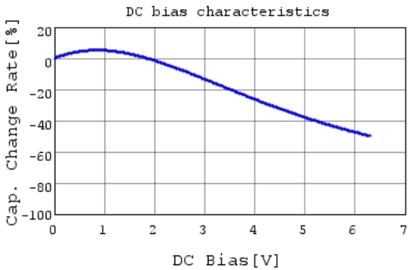
GCM31CR70J226ME23 C-DC bias capchange, 25.0c
