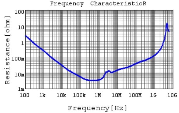
GCM31CR70J226ME23 R DC0V, 25degC
