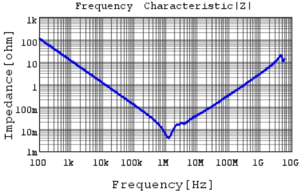
GCM31CR70J226ME23 |Z| DC0V, 25degC
