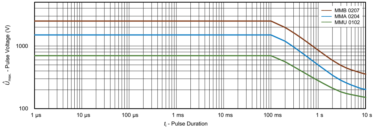
Maximum pulse voltage, single and continuous pulses; applicable if \hat{P} \leq \hat{P}_{max.} ; for permissible resistance change \pm (0.5 \% R + 0.01 \Omega)
