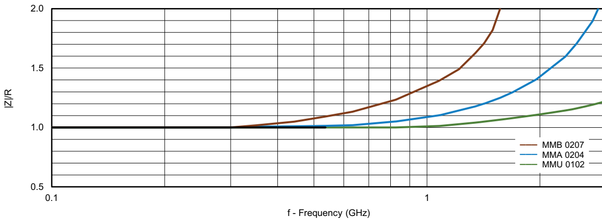
|Z|/R for 49.9 \Omega MELF resistors
