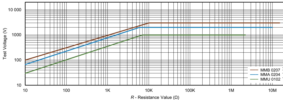
Pulse load rating in accordance with EN 60115-1 clause 8.2; 1.2 μs / 50 μs; 5 pulses at 12 s intervals; for permissible resistance change \pm (0.5 \% R + 0.05 \Omega)
