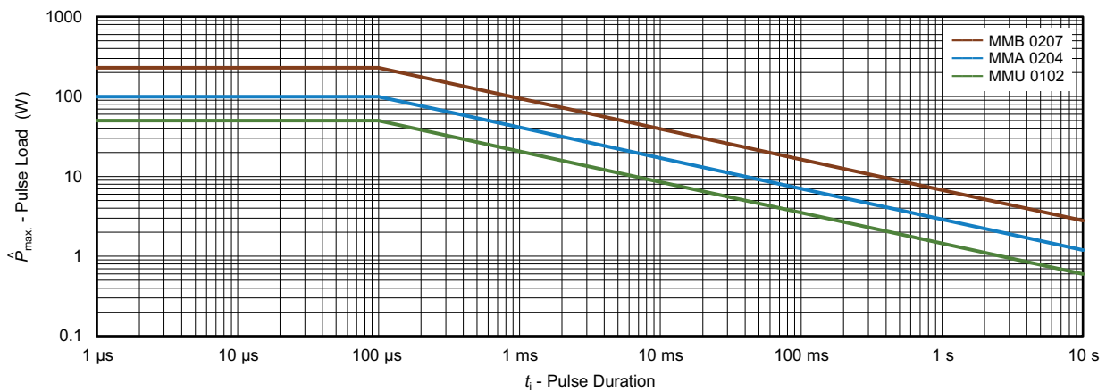
Maximum pulse load, single pulse; applicable if \bar{P} \rightarrow 0 and n \leq 1000 and \hat{U} \leq \hat{U}_{max.} ; for permissible resistance change \pm (0.5 \% R + 0.01 \Omega)
