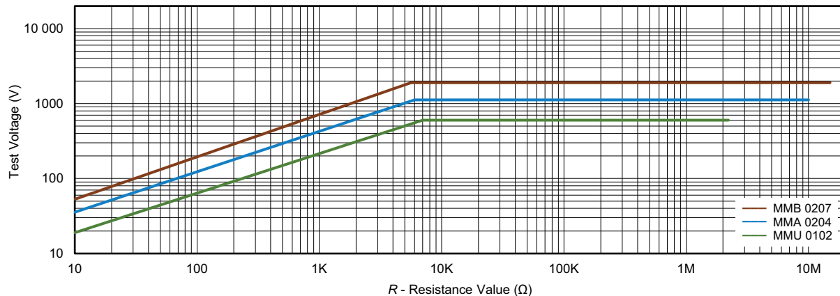
Pulse load rating in accordance with EN 60115-1 clause 8.2; 10 μs / 700 μs; 10 pulses at 1 minute intervals; for permissible resistance change \pm (0.5 \% R + 0.05 \Omega)
