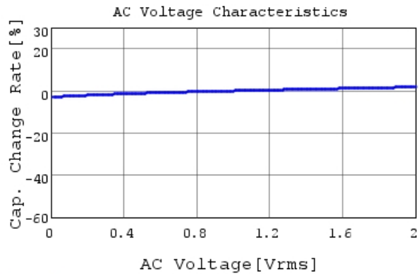
GRM216R71H103KA01 C-AC Voltage capchange, Dc
