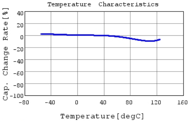
GRM216R71H103KA01 C-Temp. capchange, DC0.0V,
