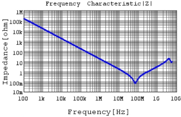
GRM216R71H103KA01 |Z| DCOV, 25degC
