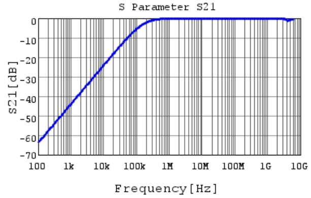
GRM216R71H103KA01 S21 DC0V, 25degC
