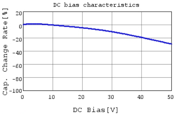
GRM216R71H103KA01 C-DC bias capchange, 25.0c
