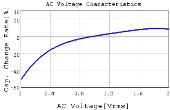
GRM155R70J105KA12 C-AC Voltage capchange, Dc
