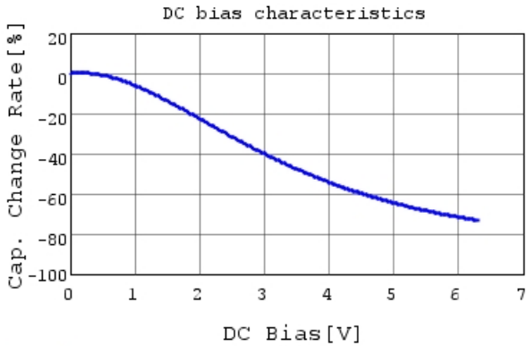
GRM155R70J105KA12 C-DC bias capchange, 25.0c
