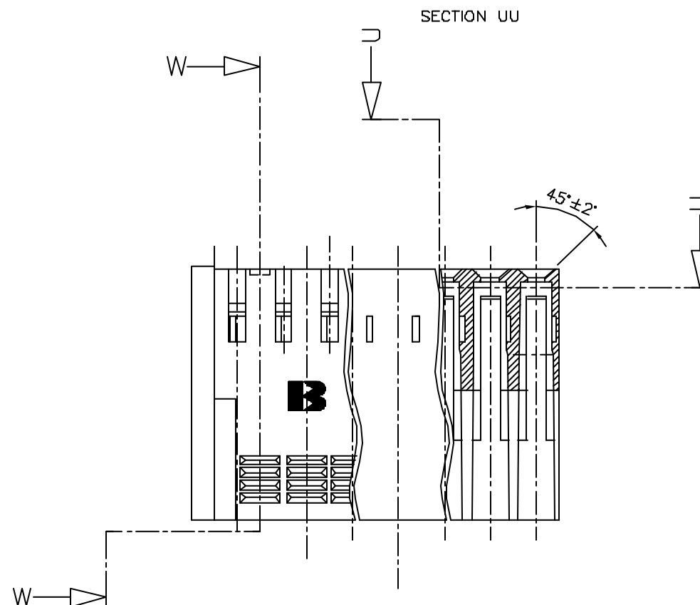
SECTION UU
