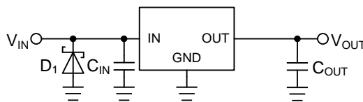
Figure 54. Surges Lower than -0.3 V will be Applied to the Input
