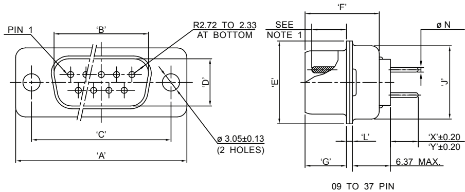
09 TO 37 PIN
