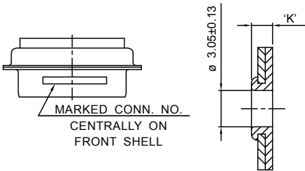
STD-THROUGH HOLE.
