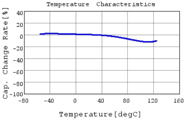
GCM216R72A103KA37 C-Temp. capchange, DC0.0V,
