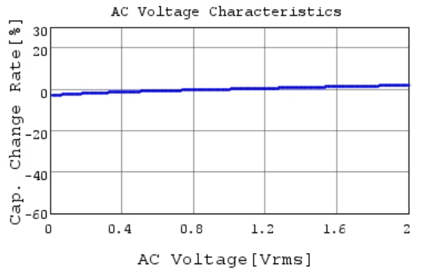
GCM216R72A103KA37 C-AC Voltage capchange, DC
