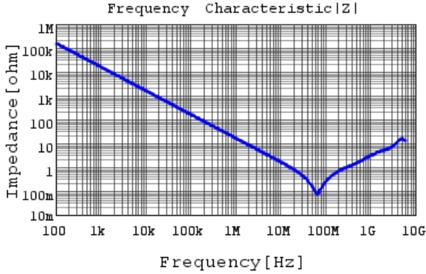
GCM216R72A103KA37 |Z| DC0V, 25degC
