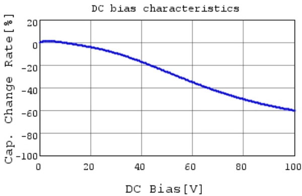
GCM216R72A103KA37 C-DC bias capchange, 25.0c
