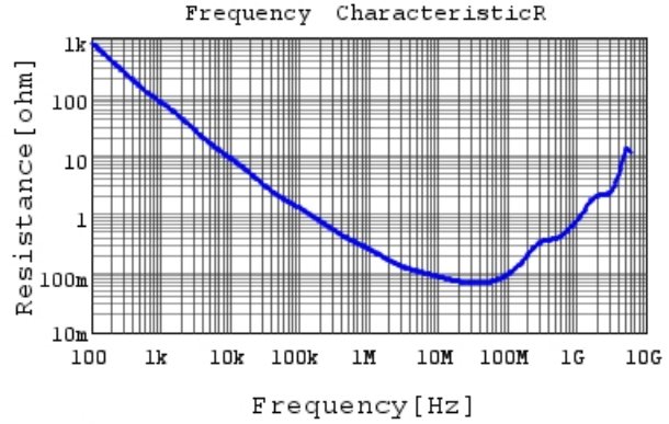
GCM216R72A103KA37 R DC0V, 25degC
