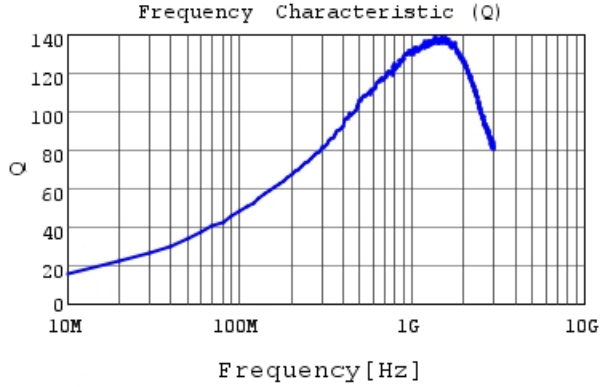
LQW2BAN12NJ00 Q
