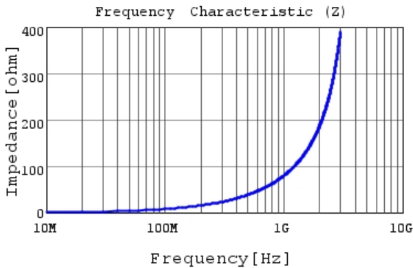
LQW2BAN12NJ00 |Z|
