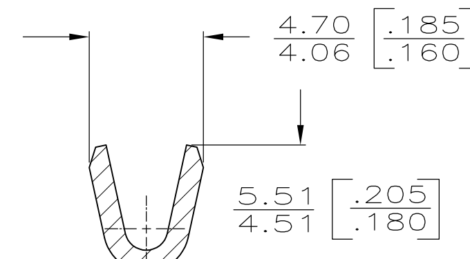
SECTION X-X
