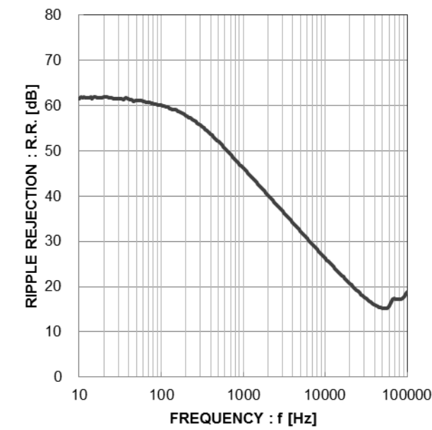
Figure 14. Ripple Rejection ( I_o=500\text{mA} )
