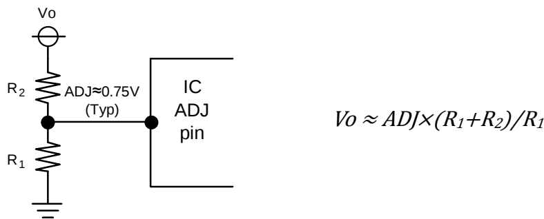
Figure 34. Output Voltage Configuration
