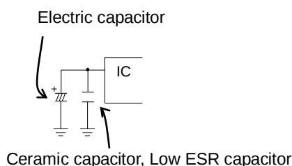
Figure 36. Input Capacitor
