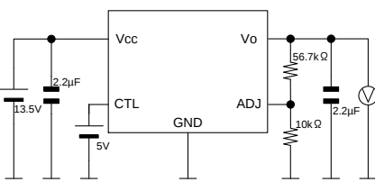
Measurement setup for Figure 15.
