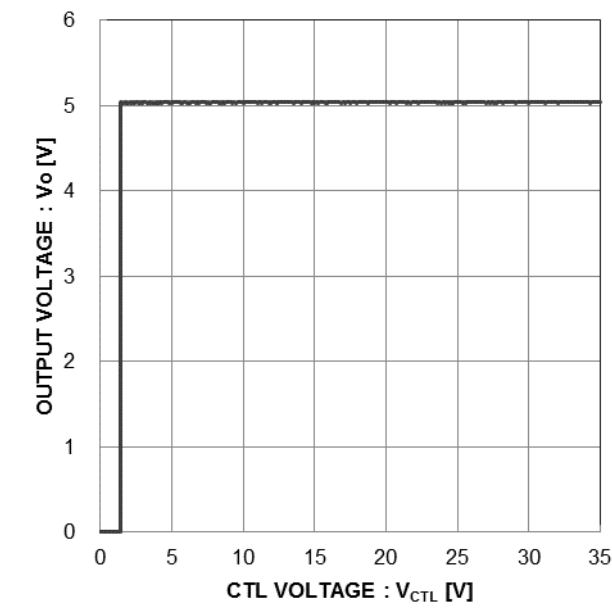
Figure 18. CTL voltage vs. Output Voltage
