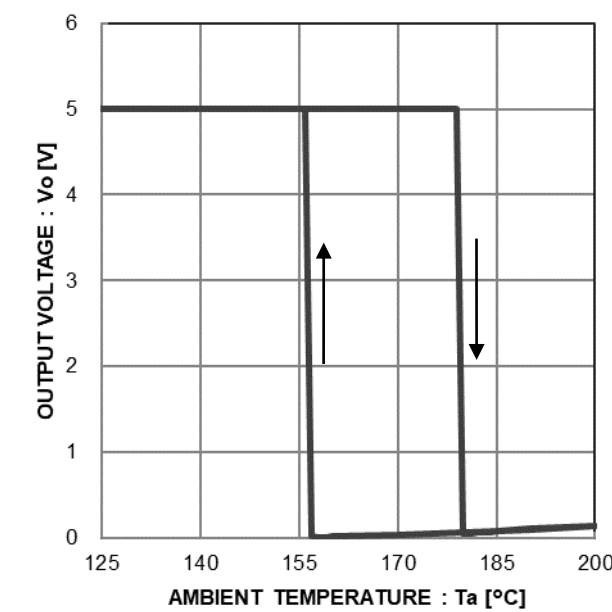
Figure 20. Thermal Shutdown Protection Characteristic
