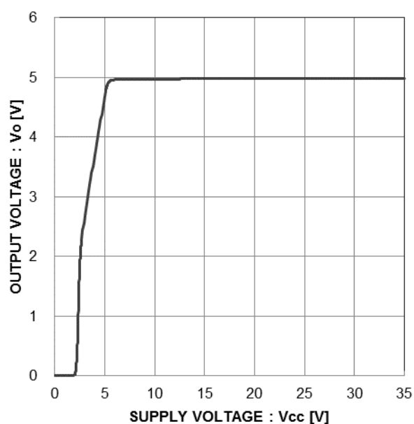
Figure 9. Line Regulation ( I_o=1.0A )
