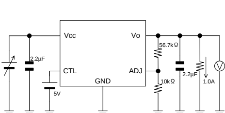
Measurement setup for Figure 9,10.
