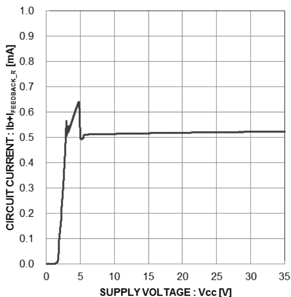
Figure 6. Circuit Current ( I_{FEEDBACK\_R} \approx 75\mu A )
