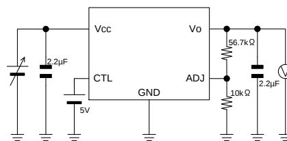
Measurement setup for Figure 8.
