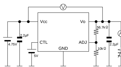
Measurement setup for Figure 13.
