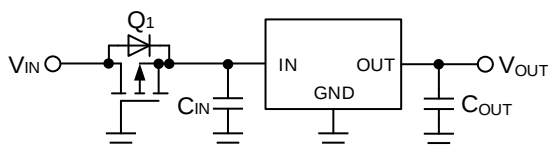
Figure 28. Protection against Reverse Polarity 2
