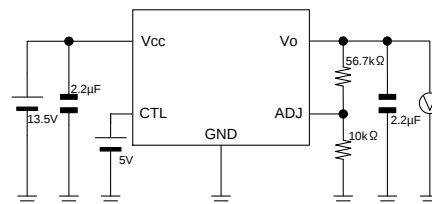
Measurement setup for Figure 20.
