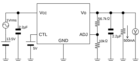
Measurement setup for Figure 14.
