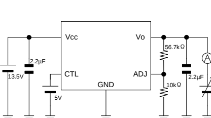
Measurement setup for Figure 11,12.
