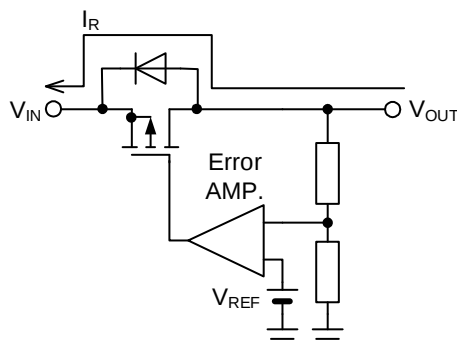
Figure 23. Reverse Current Path in an MOS Linear Regulator
