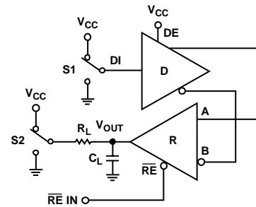
Figure 35. Receiver Enable/Disable
