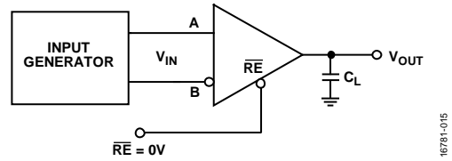
Figure 33. Receiver Propagation Delay/Skew
