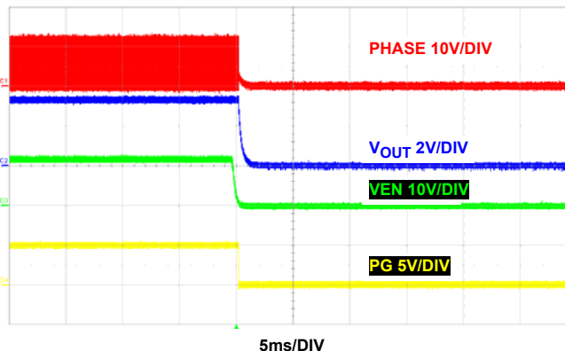
FIGURE 24. SHUTDOWN AT 300mA, PWM
