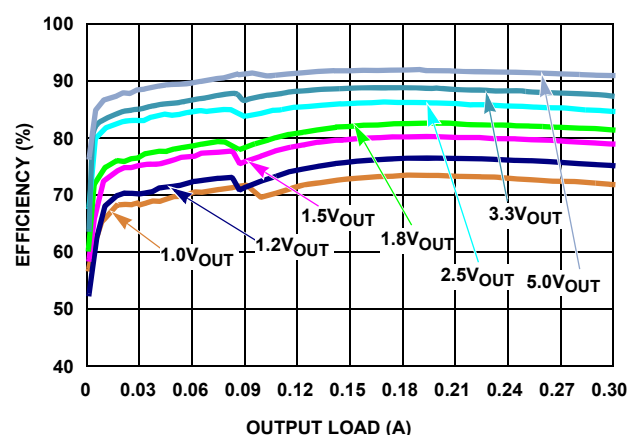
FIGURE 2. EFFICIENCY vs LOAD, PFM, V_{IN} = 12V
