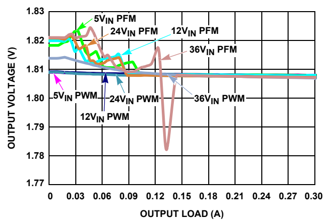
FIGURE 14. V_{OUT} REGULATION vs LOAD, V_{OUT} = 1.8\text{V}
