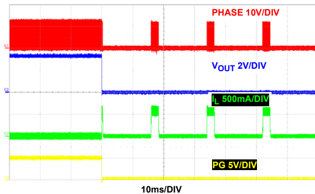
FIGURE 44. OVERCURRENT PROTECTION
