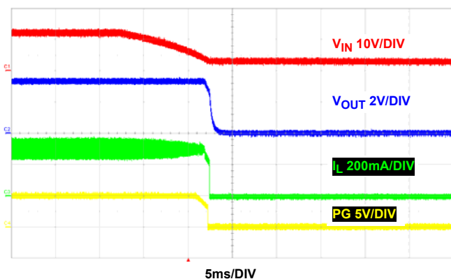
FIGURE 30. SHUTDOWN V_{IN} AT 300mA LOAD, PWM
