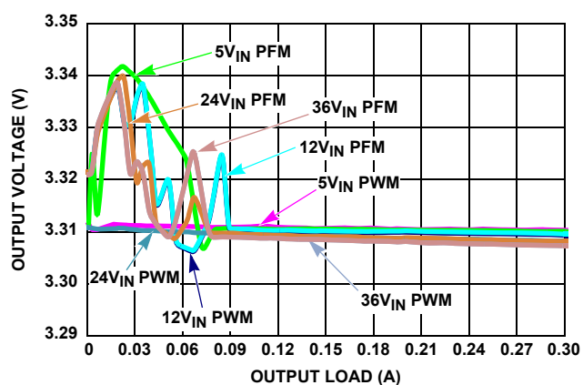
FIGURE 16. V_{OUT} REGULATION vs LOAD, V_{OUT} = 3.3\text{V}
