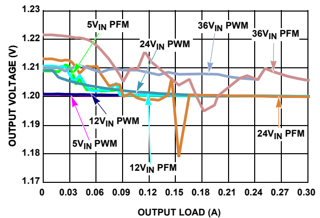
FIGURE 12. V_{OUT} REGULATION vs LOAD, V_{OUT} = 1.2\text{V}
