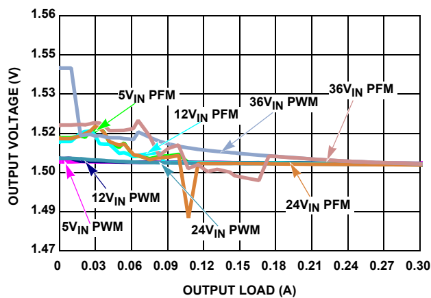
FIGURE 13. V_{OUT} REGULATION vs LOAD, PWM, V_{OUT} = 1.5\text{V}
