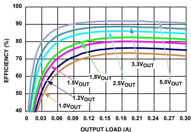
FIGURE 6. EFFICIENCY vs LOAD, PWM, V_{IN} = 12\text{V}
