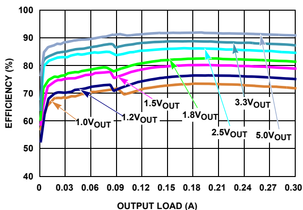
FIGURE 5. EFFICIENCY vs LOAD, PFM, V_{IN} = 12\text{V}
