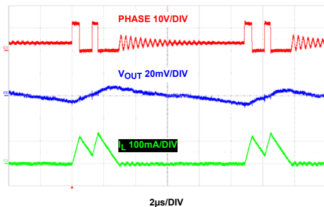
FIGURE 40. STEADY STATE AT 20mA LOAD, PFM
