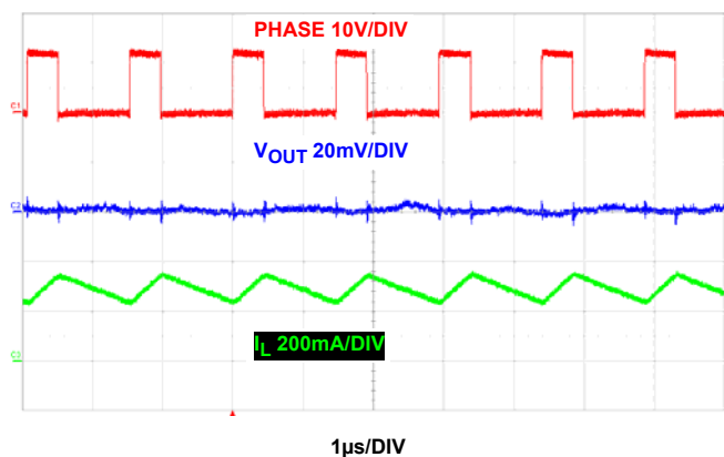
FIGURE 39. STEADY STATE AT 300mA LOAD, PWM
