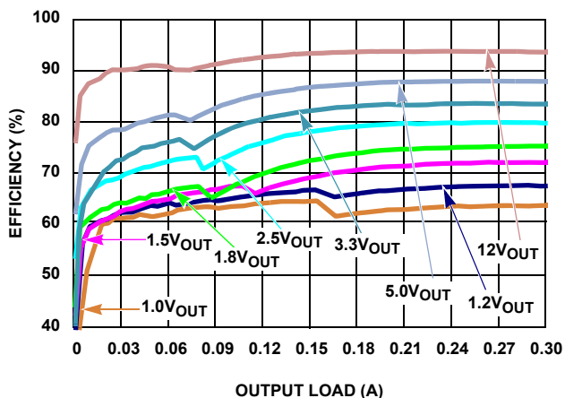
FIGURE 7. EFFICIENCY vs LOAD, PFM, V_{IN} = 24\text{V}
