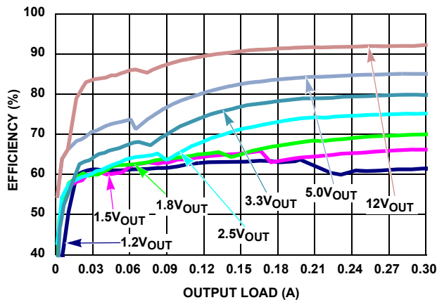
FIGURE 9. EFFICIENCY vs LOAD, PFM, V_{IN} = 36\text{V}
