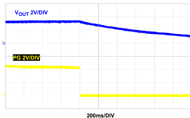
FIGURE 48. OVER-TEMPERATURE PROTECTION
