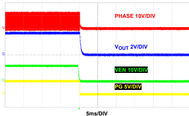
FIGURE 26. SHUTDOWN AT 300mA, PFM
