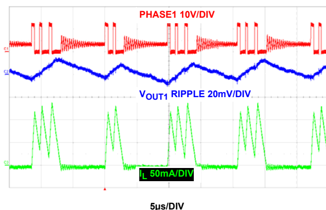
FIGURE 46. PWM TO PFM TRANSITION
