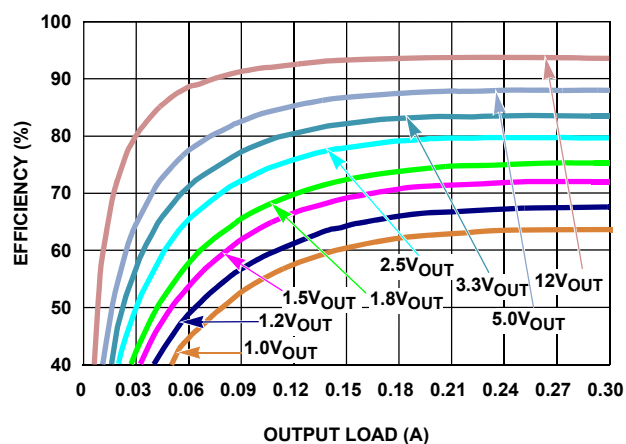
FIGURE 8. EFFICIENCY vs LOAD, PWM, V_{IN} = 24\text{V}
