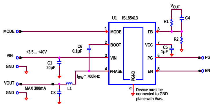
FIGURE 1. TYPICAL APPLICATION
