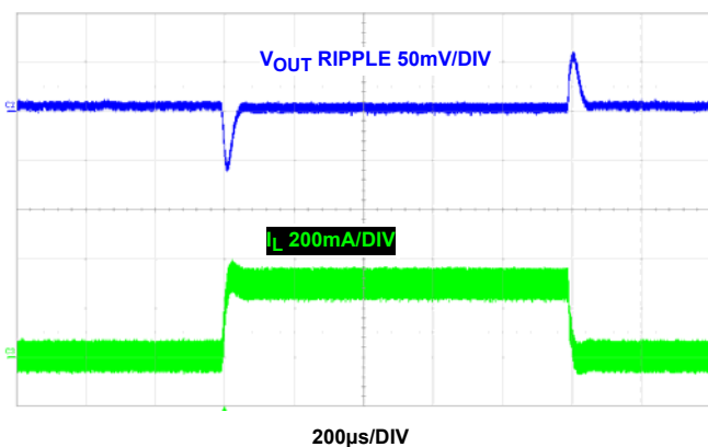
FIGURE 42. LOAD TRANSIENT, PWM
