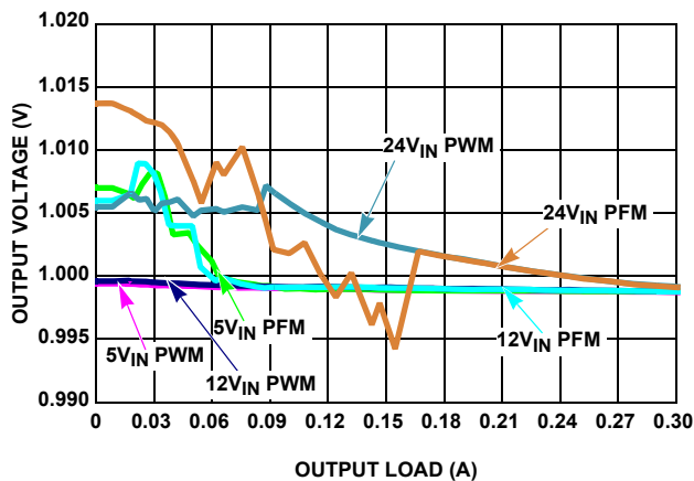
FIGURE 11. V_{OUT} REGULATION vs LOAD, V_{OUT} = 1\text{V}
