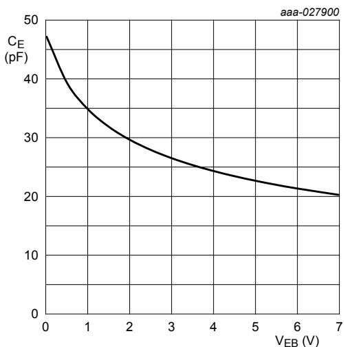
f = 1\text{ MHz}; T_{amb} = 25\text{ }^{\circ}\text{C} Figure 29. BC817K-25H: Emitter capacitance as a function of emitter-base voltage; typical values
