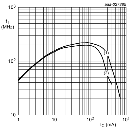
f = 100\text{ MHz}; T_{amb} = 25\text{ }^{\circ}\text{C} (1) V_{CE} = 5\text{ V} (2) V_{CE} = 1\text{ V} Figure 30. BC817K-25H: Transition frequency as a function of collector current voltage; typical values
