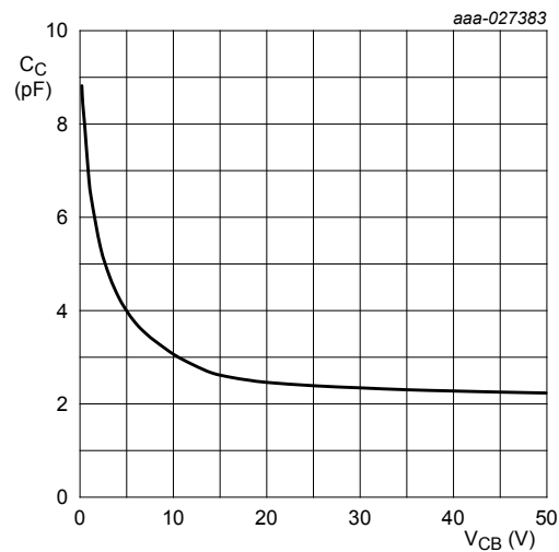
f = 1\text{ MHz}; T_{amb} = 25\text{ }^{\circ}\text{C} Figure 28. BC817K-25H: Collector capacitance as a function of collector-base voltage; typical values
