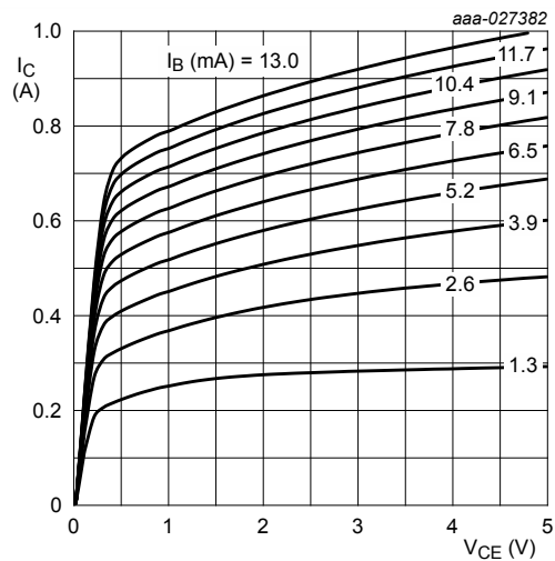
T_{amb} = 25\text{ }^{\circ}\text{C} Figure 27. BC817K-25H: Collector current as a function of collector-emitter voltage; typical values
