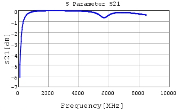
GCM1555C1H9R0BA16 S21 DCOV, 25degC
