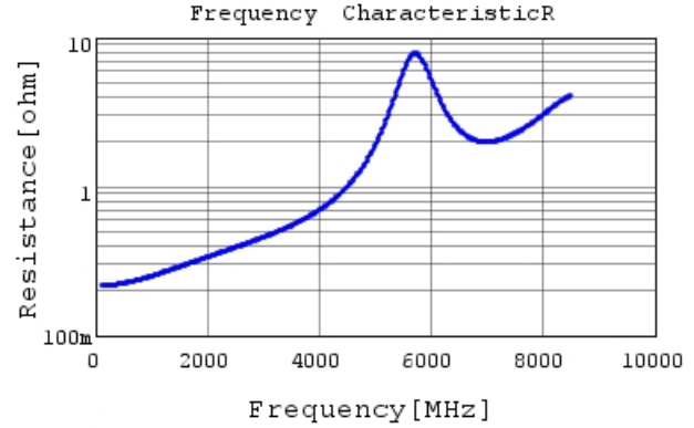
GCM1555C1H9R0BA16 R DCOV, 25degC
