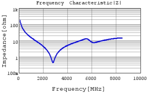
GCM1555C1H9R0BA16 |Z| DCOV, 25degC
