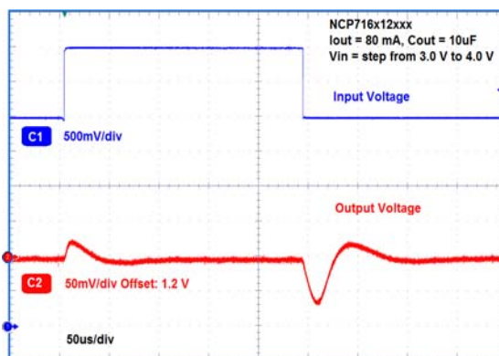
Figure 34. Line Transient Response
