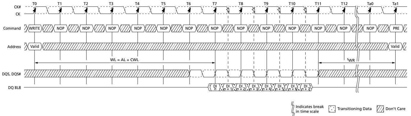
Figure 89: WRITE (BL8) to PRECHARGE
