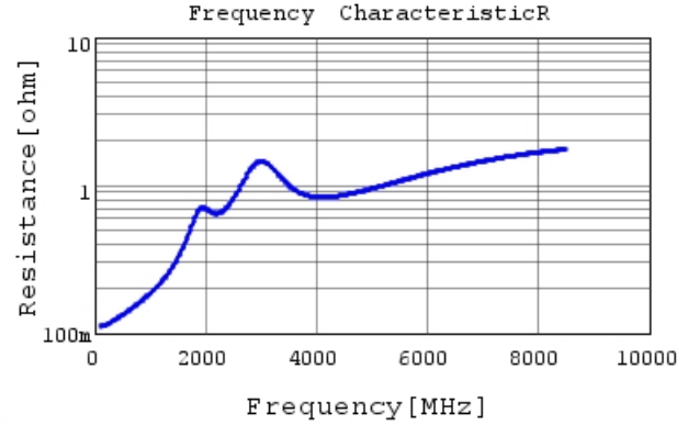
GRT1555C1H101JA02 R DCOV,25degC
