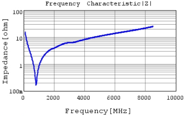
GRT1555C1H101JA02 |Z| DCOV,25degC
