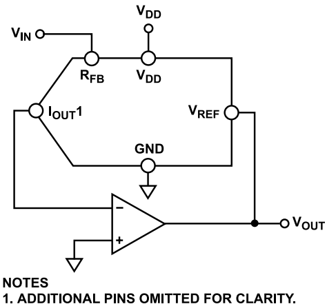
Figure 42. Current-Steering DAC Used as a Divider or Programmable Gain Element
