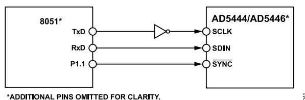
Figure 49. 80C51/80L51 to AD5444/AD5446 Interface
