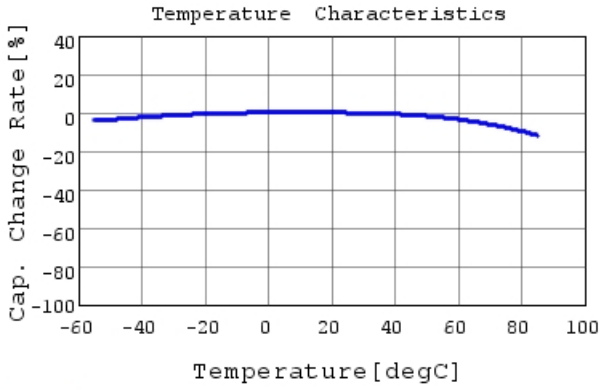
GRM319R6YA106KA12 C-Temp. capchange, DC0.0V,
