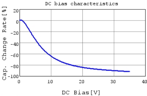
GRM319R6YA106KA12 C-DC bias capchange, 25.0c
