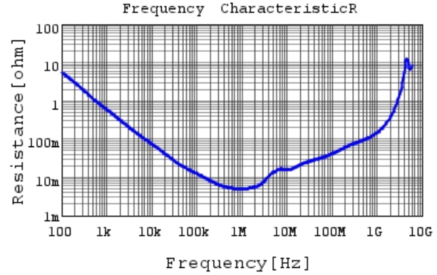
GRM319R6YA106KA12 R DCOV, 25degC
