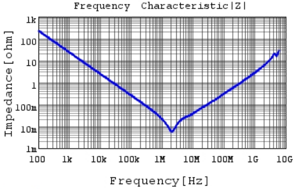
GRM319R6YA106KA12 |Z| DCOV, 25degC
