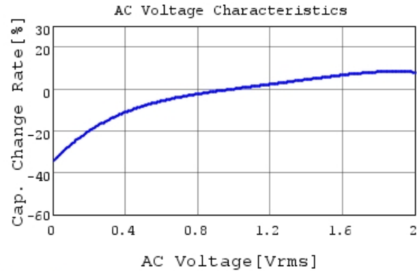
GRM319R6YA106KA12 C-AC Voltage capchange, Dc
