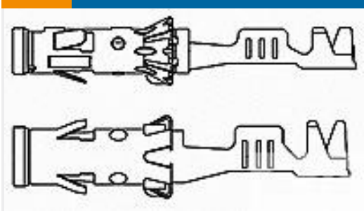
TE Part #929989-7 1,5MM CONT.SOCK SWS
