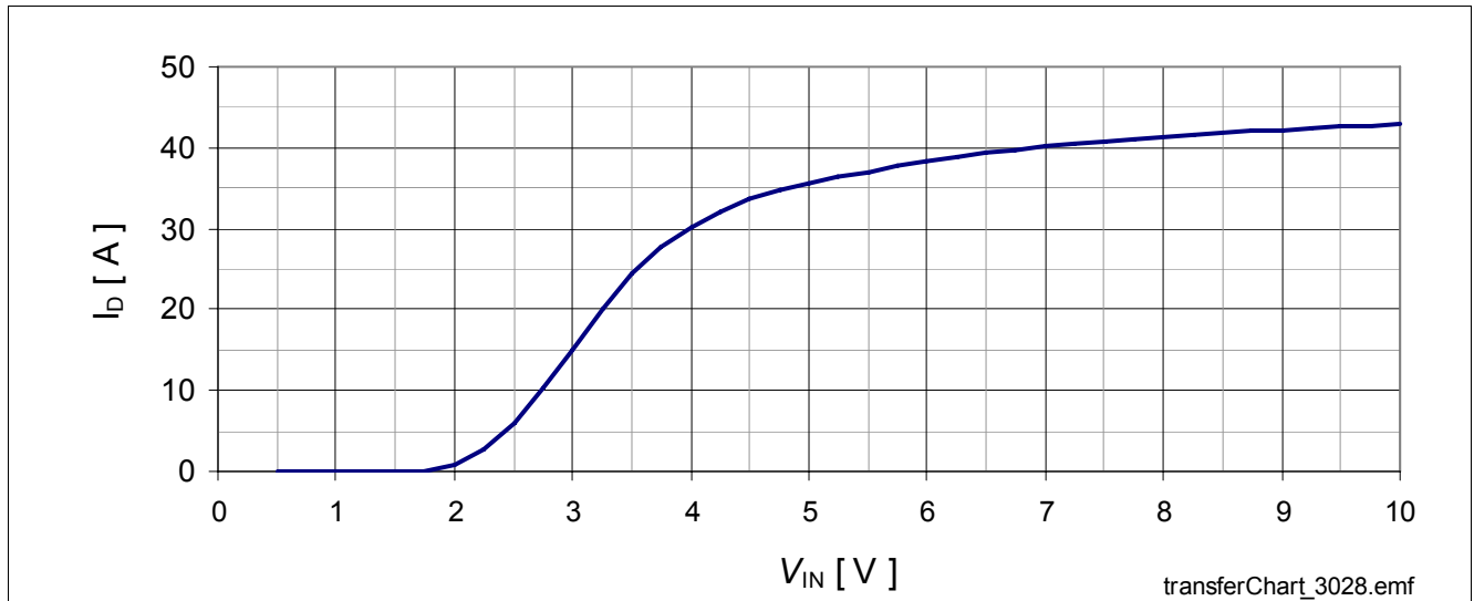
Figure 7 Typical Transfer Characteristic I_D = f(V_{IN}) ; V_D = 13.5 \text{ V} , T_{J(\text{start})} = 25 \text{ °C}
