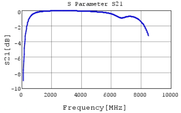
GRM1885C1H6R0CA01 S21 DCOV, 25degC
