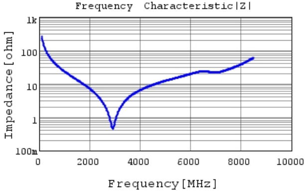
GRM1885C1H6R0CA01 |Z| DCOV, 25degC
