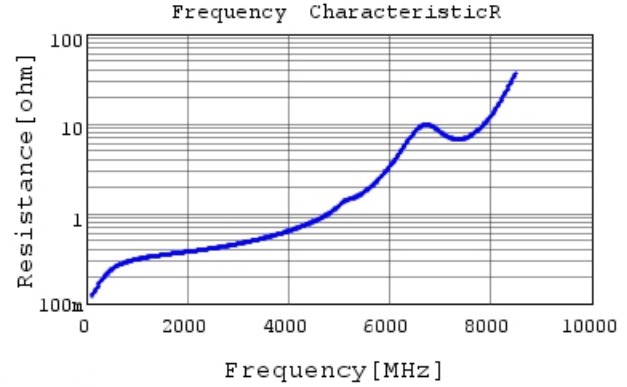
GRM1885C1H6R0CA01 R DCOV, 25degC
