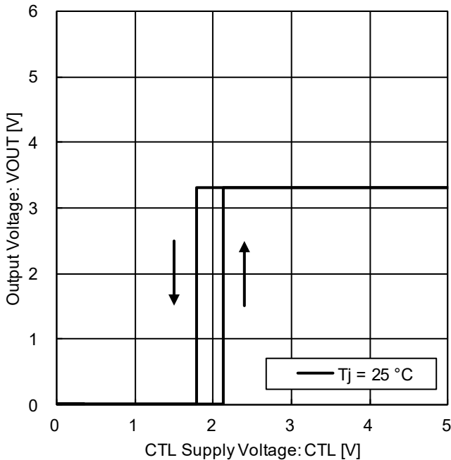
Figure 18. CTL ON / OFF Mode Voltage ( T_j = 25\text{ °C} )
