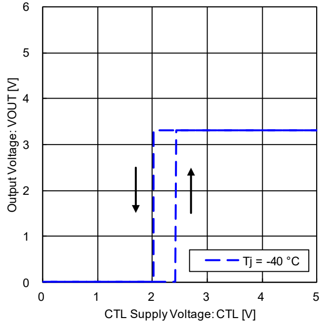
Figure 17. CTL ON / OFF Mode Voltage ( T_j = -40\text{ °C} )
