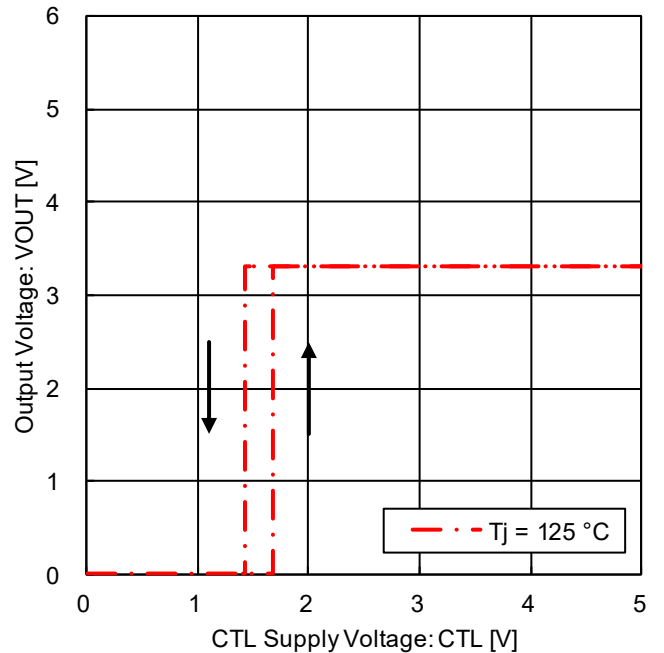
Figure 19. CTL ON / OFF Mode Voltage ( T_j = 125\text{ °C} )
