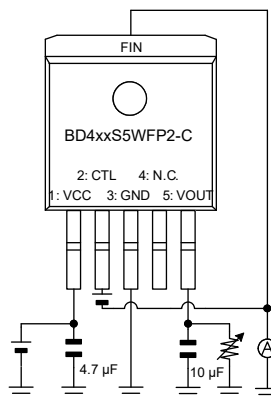
Measurement Setup for Figure 12, 30
