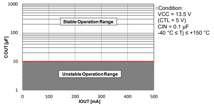
Figure 41. COU (Typ) vs IOU
