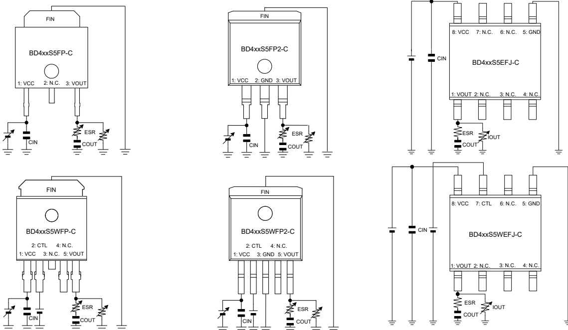
Figure 42. Measurement Setups for ESR Reference Data
