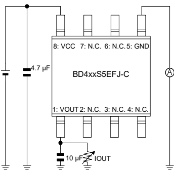
Measurement Setup for Figure 12, 30
