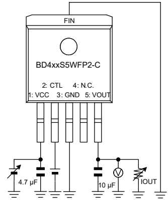
Measurement Setup for Figure 8, 26
