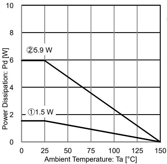
Figure 54. Package Data (TO263-3 / TO263-5)
