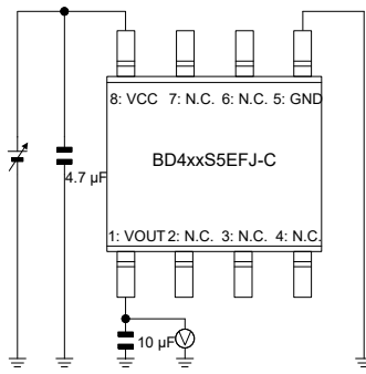
Measurement Setup for Figure 5, 7, 13, 14, Figure 23, 25, 31, 32
