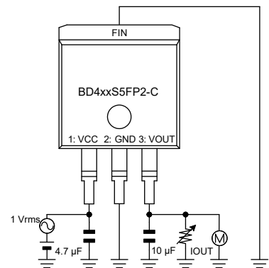
Measurement Setup for Figure 11, 29
