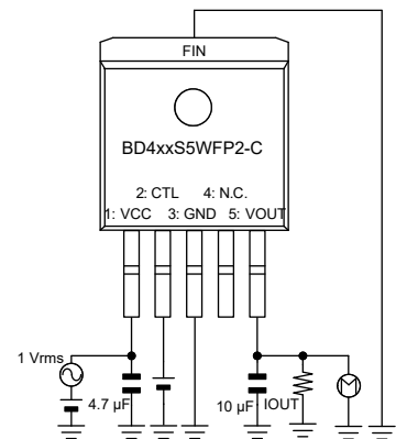
Measurement Setup for Figure 11, 29
