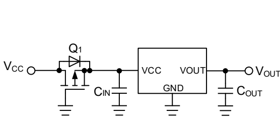
Figure 50. Protection against Reverse Polarity 2
