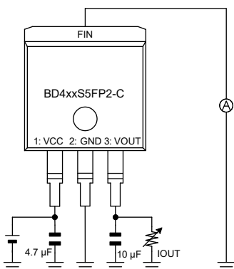
Measurement Setup for Figure 12, 30
