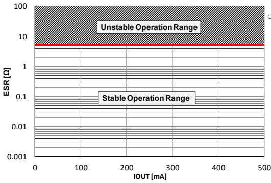
Figure 40. ESR vs IOU
