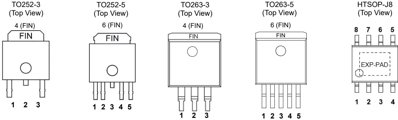
Figure 3. Pin Configurations
