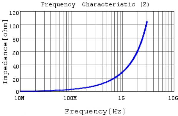
LQG15HN4N7B02 |Z|
