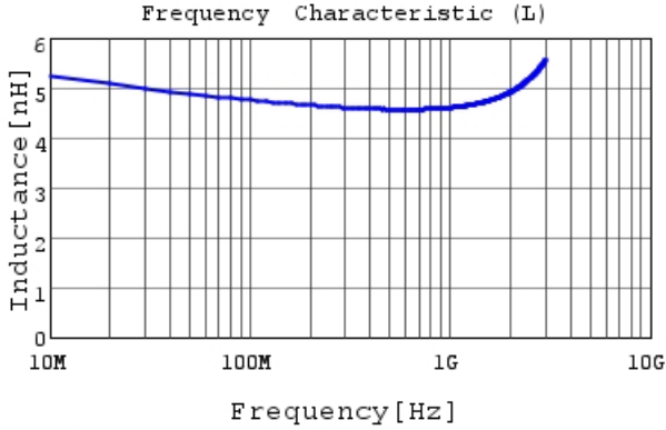
LQG15HN4N7B02 L
