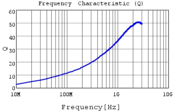
LQG15HN4N7B02 Q
