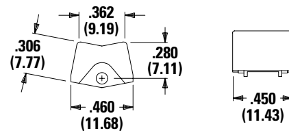
J60 Lever
