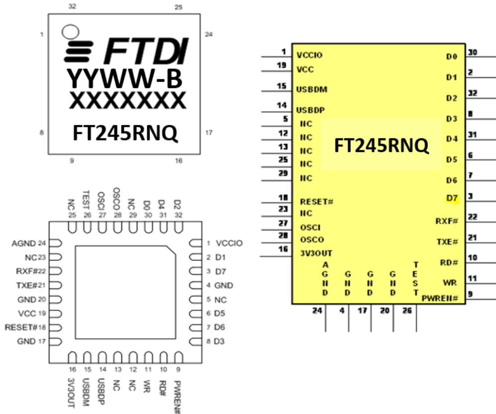
Figure 3.2 QFN-32 Package Pin Out and schematic symbol
