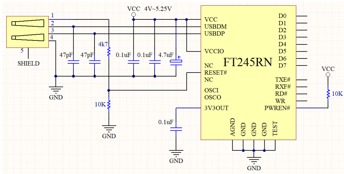
Figure 6.2 Self-Powered Configuration
