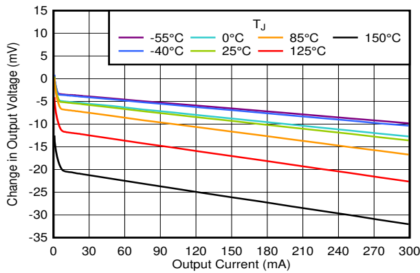
Figure 5-7. Load Regulation vs I_{OUT} V_{IN} = 2.8 \text{ V} , V_{EN} = 1 \text{ V} , DBV package
