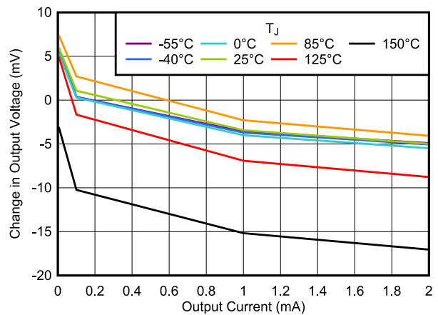
Figure 5-12. Load Regulation vs I_{OUT} V_{OUT} = 5.5 \text{ V} , V_{EN} = 1 \text{ V} , DBV package
