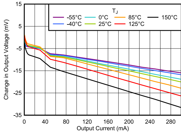
Figure 5-7. Load Regulation vs I_{OUT} V_{IN} = 2.8 \text{ V} , V_{EN} = 1 \text{ V} , DBV package
