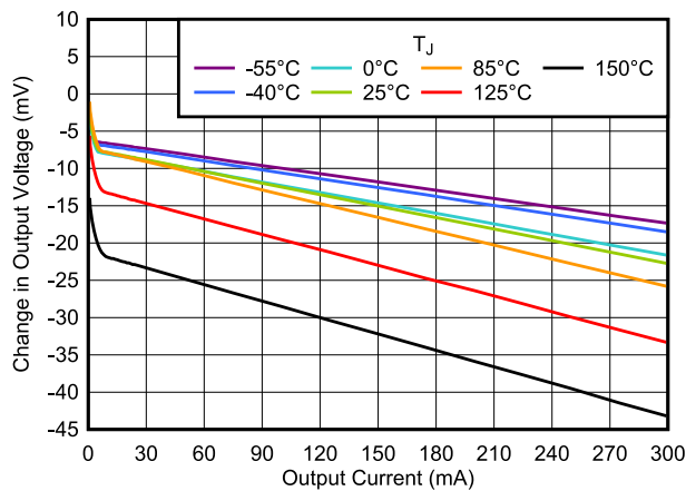
Figure 5-11. Load Regulation vs I_{OUT} V_{OUT} = 5.5 \text{ V} , V_{EN} = 1 \text{ V} , DBV package
