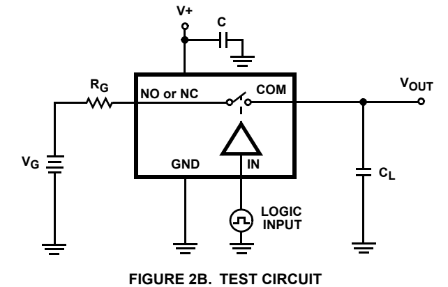
FIGURE 2. CHARGE INJECTION
