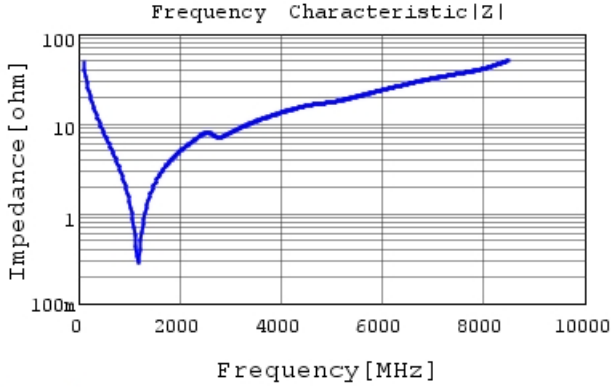
GRM1885C1H330JA01 |Z| DCOV, 25degC
