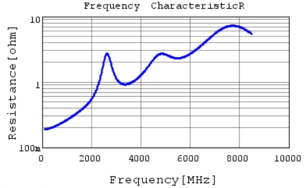
GRM1885C1H330JA01 R DCOV, 25degC
