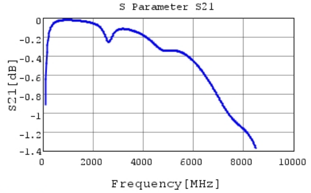
GRM1885C1H330JA01 S21 DCOV, 25degC
