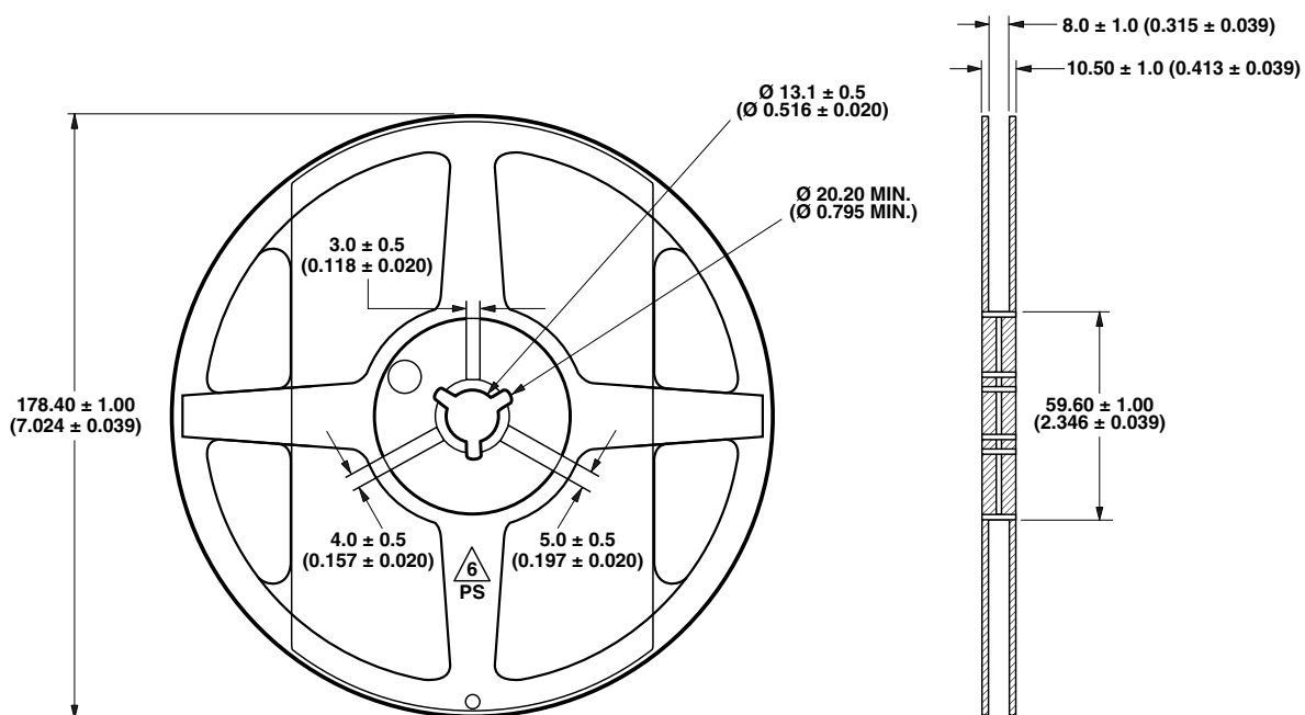
Figure 15. Reel dimensions.
