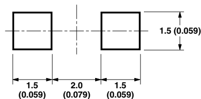
Figure 13. Recommended soldering pattern for HSMx-C150.
