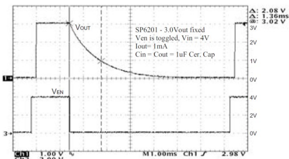
Fig. 26: Turn off time, I_O=1\text{mA} , 4V_{IN}
