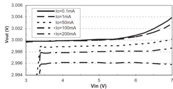
Fig. 18: Line Regulation (SP6201 fixed 3.0V)
