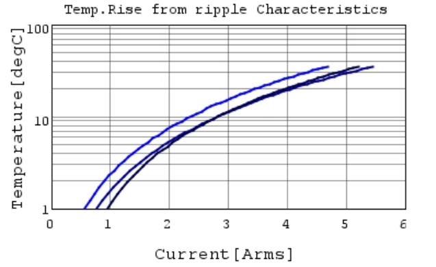
GRM188R60G226MEA0 Temp.rise — 80kHz
