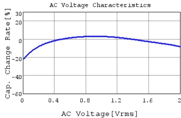
GRM188R60G226MEA0 C-AC Voltage capchange, Dc
