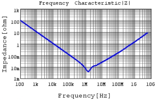
GRM188R60G226MEA0 |Z| DCOV, 25degC
