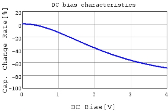
GRM188R60G226MEA0 C-DC bias capchange, 25.0c
