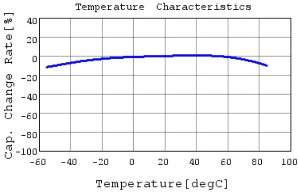
GRM188R60G226MEA0 C-Temp. capchange, DCO.0V,
