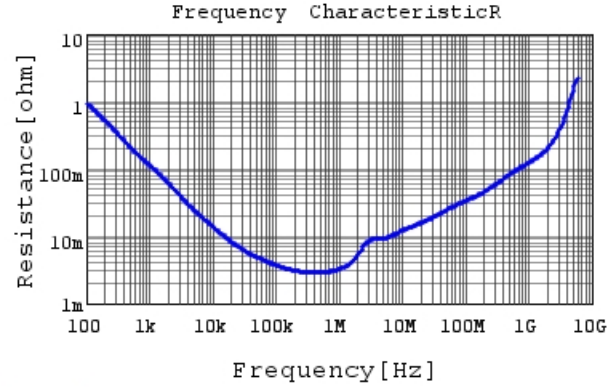
GRM188R60G226MEA0 R DCOV, 25degC
