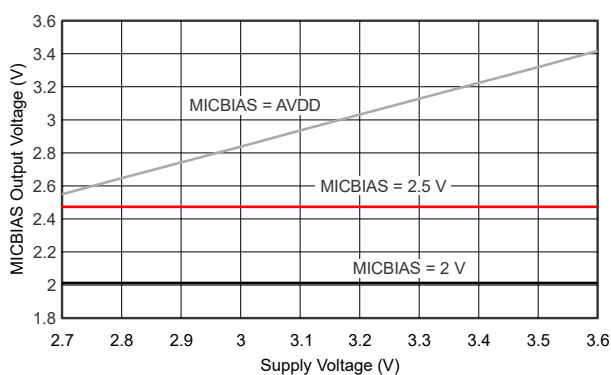
Figure 6-9. MICBIAS Output Voltage vs AVDD
