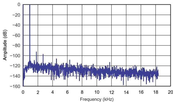
Figure 9-2. DAC to Line Output FFT at 1-kHz Signal Plot
