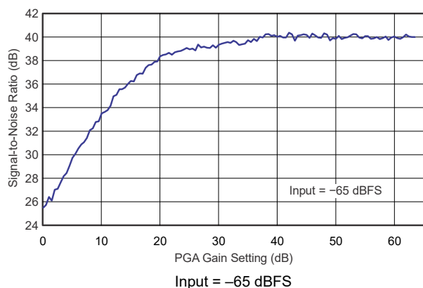
Figure 6-7. ADC SNR vs PGA Gain Setting, -65-dBFS Input
