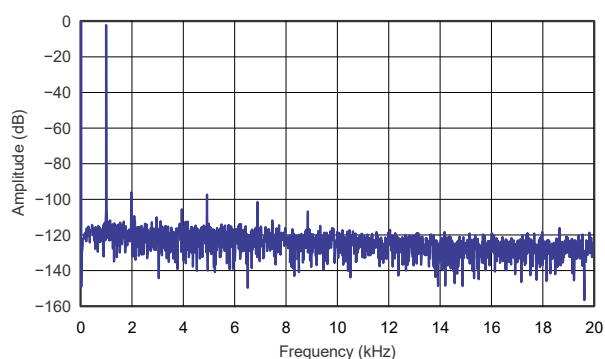
Figure 6-6. Line Input to ADC FFT Plot
