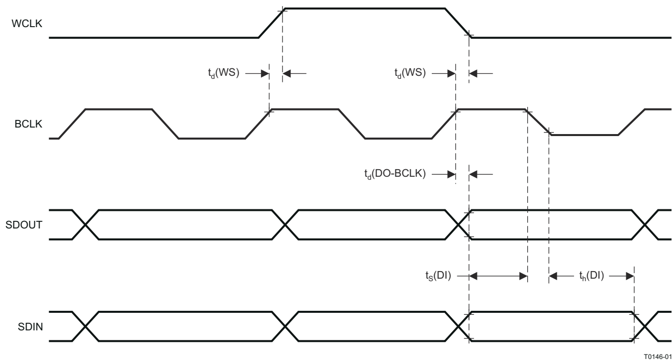
Figure 6-3. DSP Timing in Master Mode
