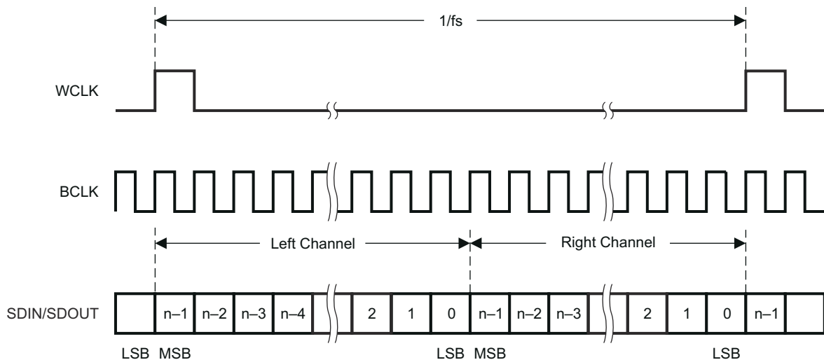
Figure 7-19. DSP Serial Data Bus Mode Operation
