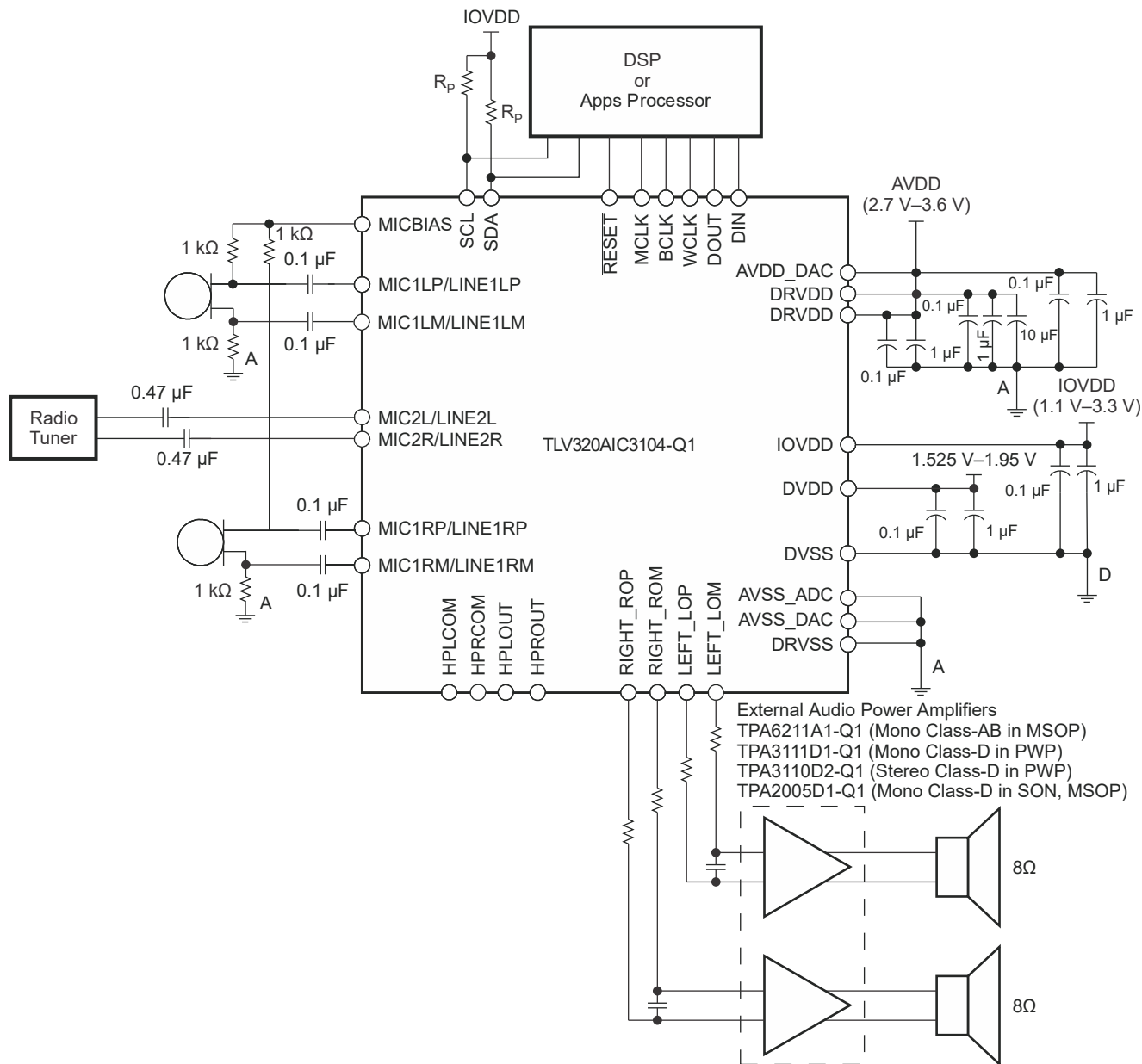
Figure 9-1. Typical Connections With Differential Inputs for External Speaker Driver
