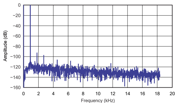
Figure 6-5. DAC to Line Output FFT Plot
