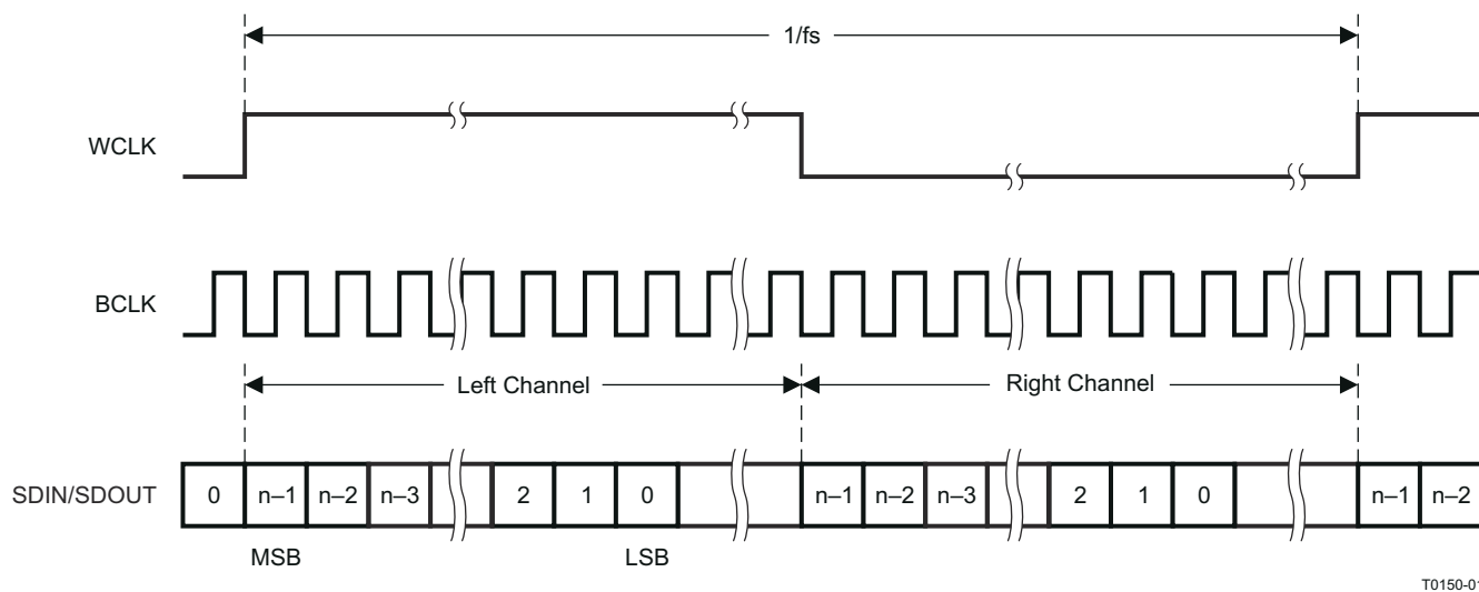
Figure 7-17. Left-Justified Serial Data Bus Mode Operation
