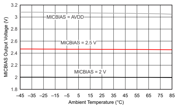
Figure 6-10. MICBIAS Output Voltage vs Ambient Temperature
