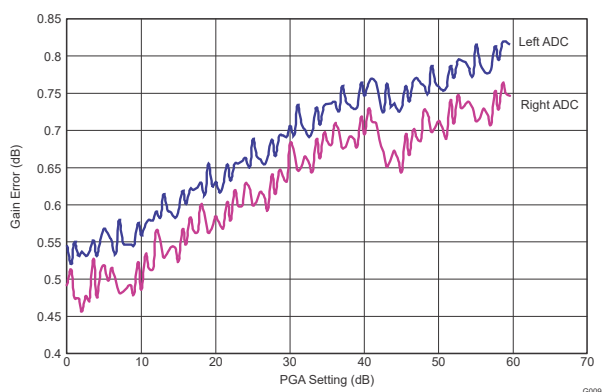
Figure 6-8. ADC Gain Error vs PGA Gain Setting
