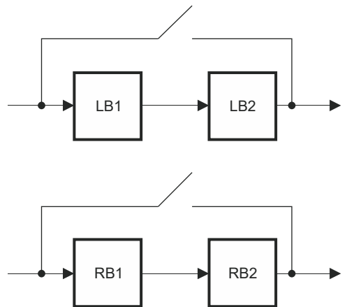
Figure 7-2. Structure of Digital Effects Processing for Channel Processing
