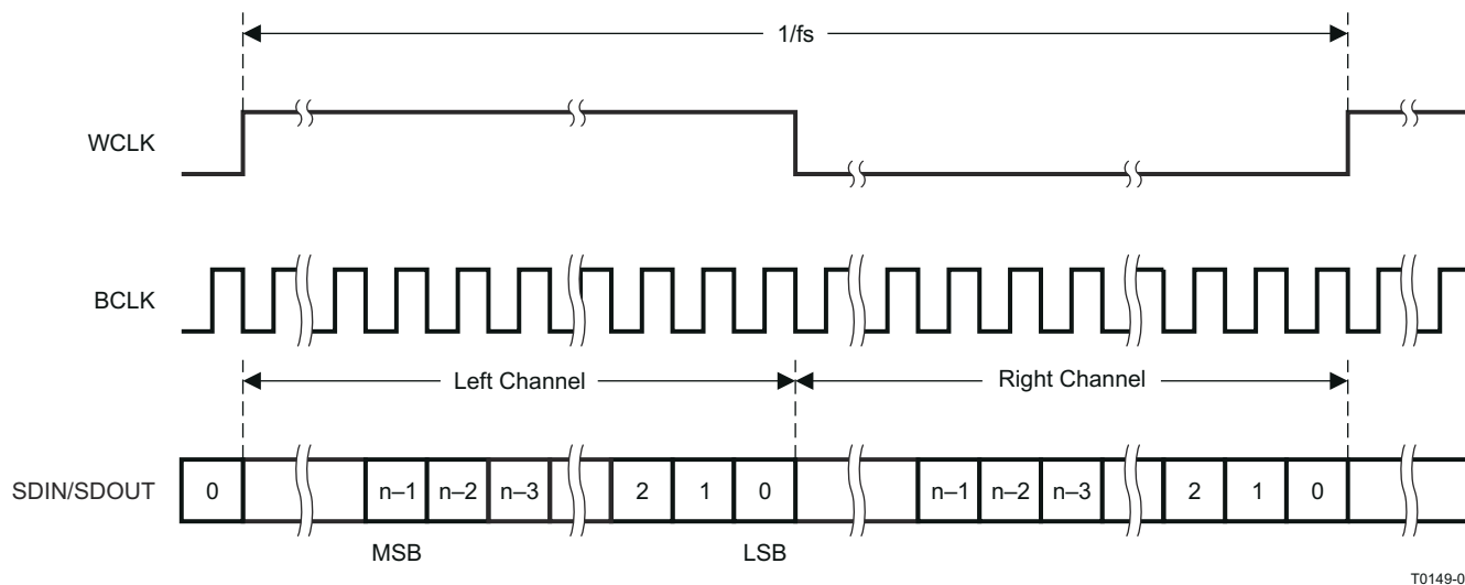
Figure 7-16. Right-Justified Serial Data Bus Mode Operation
