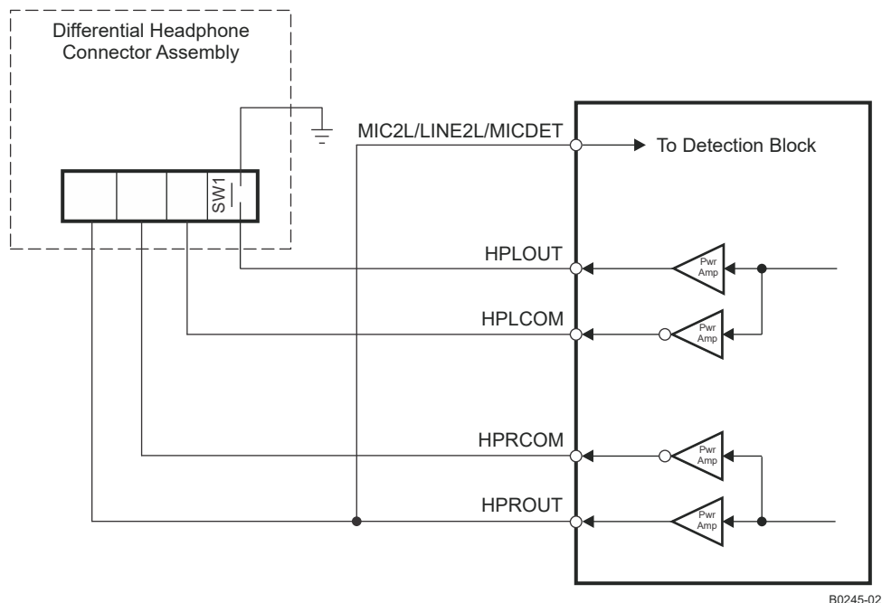
Figure 7-10. Configuration of Device for Jack Detection Using Fully-Differential Stereo Headphone Output Connection
