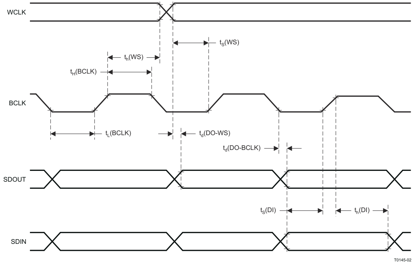
Figure 6-2. I²S/LJF/RJF Timing in Slave Mode
